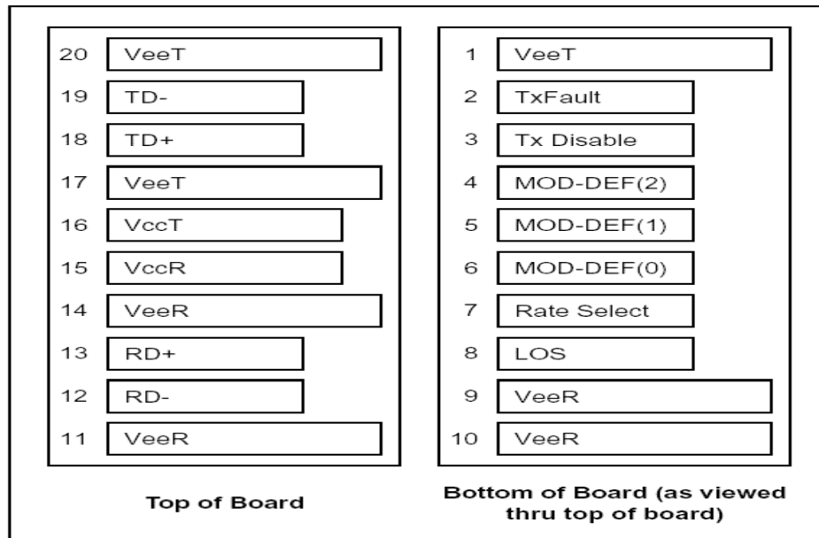
Figure 1. Pin Definitions
