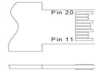
TOP VIEW OF BOARD
