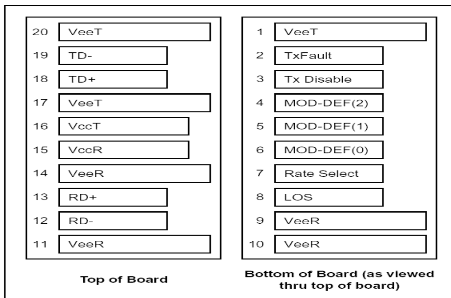
Figure 1. Pin Definitions
