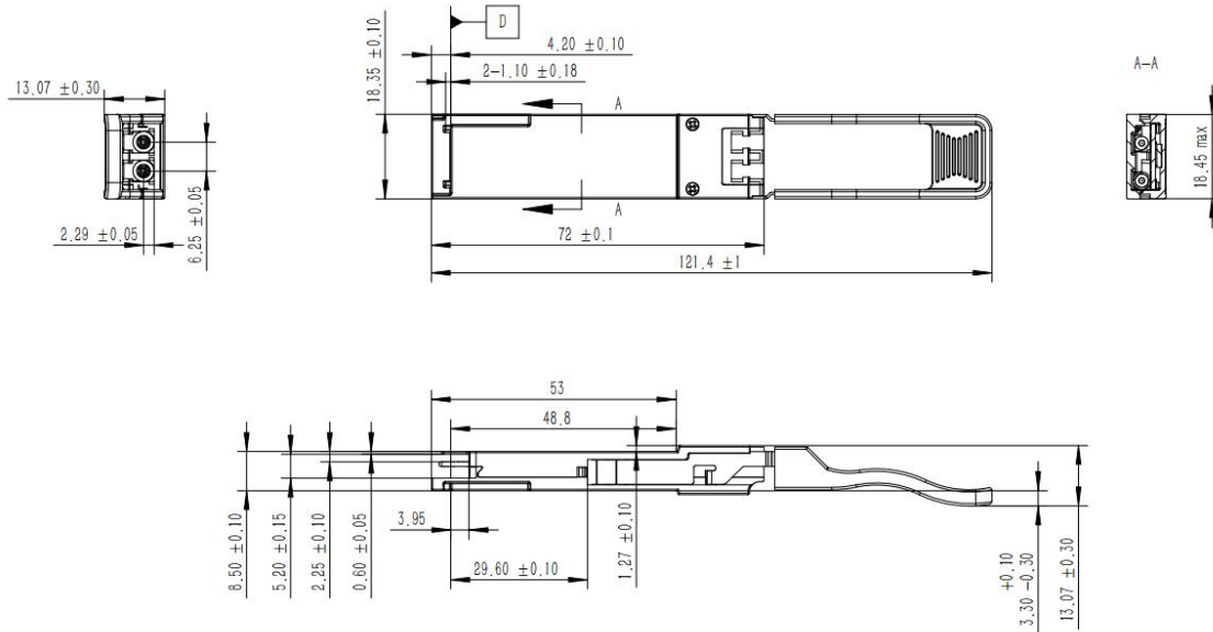
Figure 2. Mechanical dimensions
