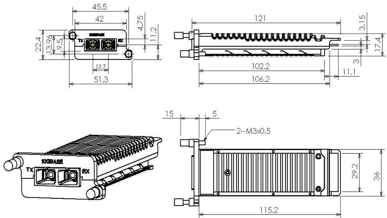
Figure 1 Mechanical dimensions
